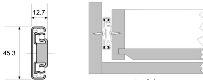
Installation Diagram
