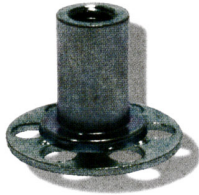
Zinc plated Mild Steel female threaded insert on a blind 23mm diameter base plate
