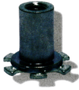
Zinc plated Mild Steel female threaded insert on a blind 19mm diameter base plate
