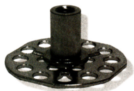
316 Stainless Steel female threaded insert on a blind 38mm diameter base plate
